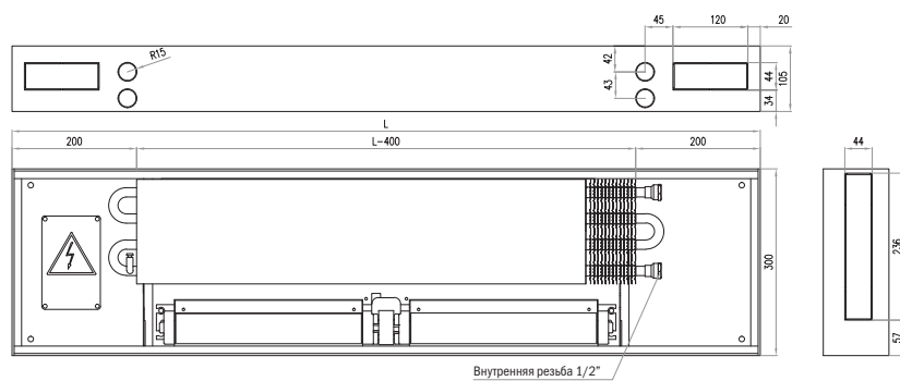
TKV-13 Lx30x10
