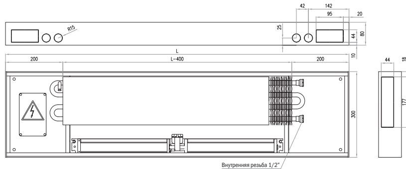
TKV-13 Lx30x10
