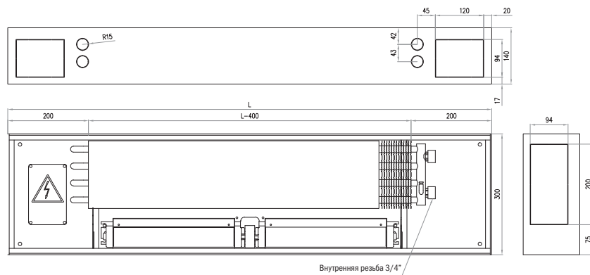
TKV-13 Lx30x14
